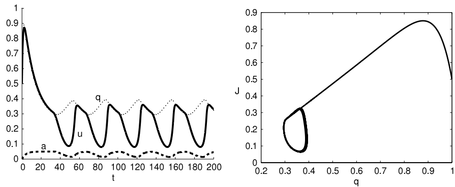
Fig. 11. Numerical simulation of the space-clamped system (5.1) using the parameters \tau = 0.01 , \kappa = 4 , \alpha = 50 , \beta = 0.06 , \gamma = 4 , and \epsilon = 0.05 . (Left) Plot of u , q , and a trajectories in time. As predicted by linear stability analysis, the solution settles into a limit cycle about the Up state. (Right) A plot in the (q; J) phase plane, where J = u - a is the total current input to the firing rate function f(\cdot) . Notice that at its lowest point, J dips below the value corresponding to the mean value of f : f(J) = 0.135; 0.5 .
